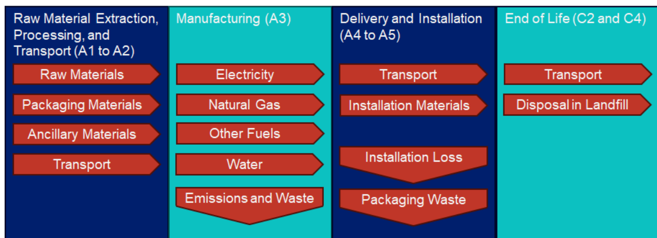
Figure 1-1: Simplified process flow diagram for 5/8" ToughRock® Fireguard C® Gypsum Board
